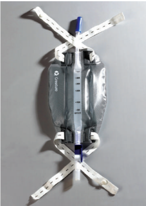
Leg Bag Ref. No.: NMU230114 (three chambers)
